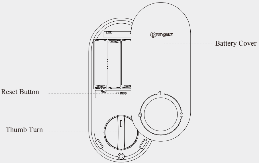
Interior Assembly
